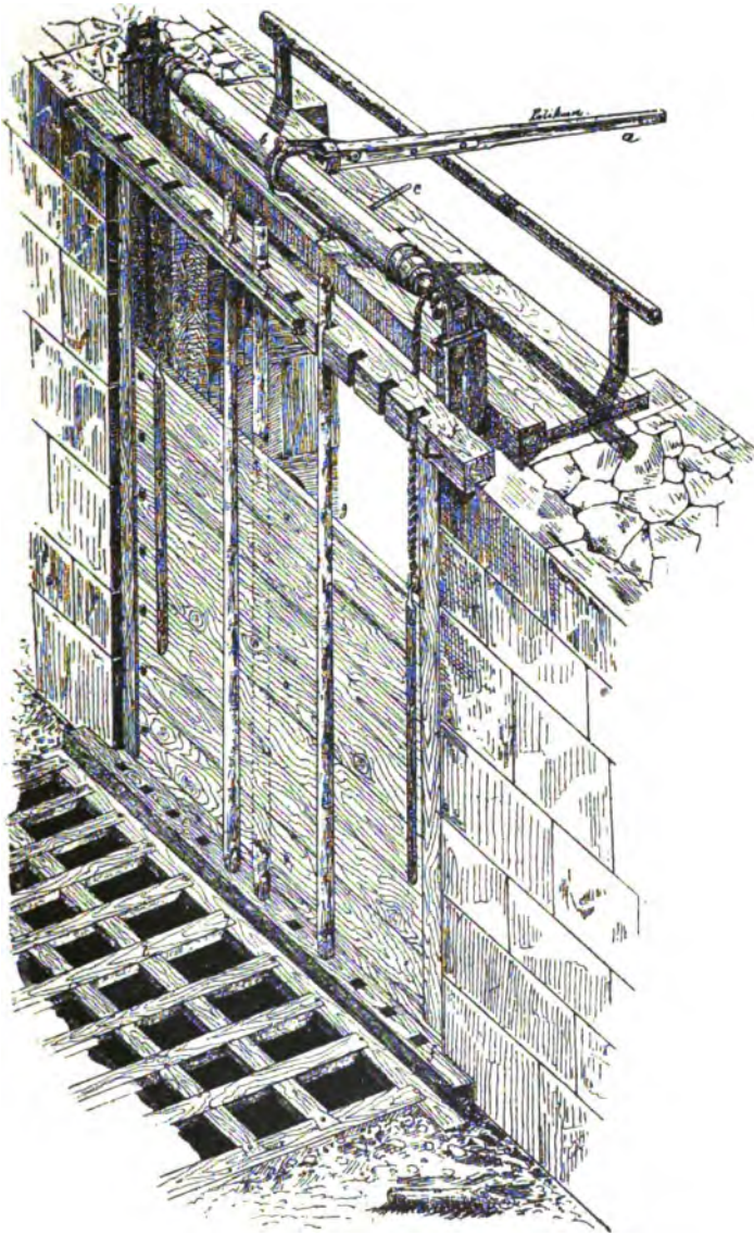
Fig. 270.—Sand-grating and sluice.*
